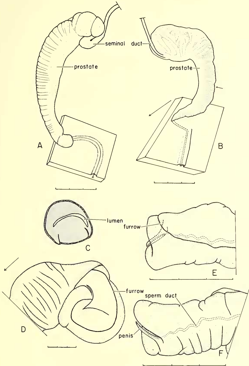
TEXT-FIG. 11. Male reproductive structures of Neocyclotus . A. N. bisinuatus (Martens), prostate; Tapanti, Costa Rica. B. N. d. ambiguum (Martens), prostate; 8.6 mi. é Chiapa de Corzo, Chiapas. C. Cross-section through prostate of B at point indicated by arrow. D-F. N. d. ambiguum (Martens), dorsal view of verge (D) and enlarged illustrations of dorsal (E) and ventral (F) views of the verge showing the relationships of the sperm duct to the seminal furrow and the penis. Scales equal 3 mm.
